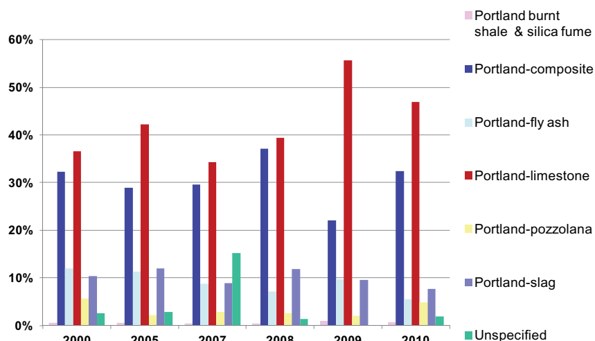
Domestic deliveries of CEM II sub-type CEMBUREAU 2000-2010
